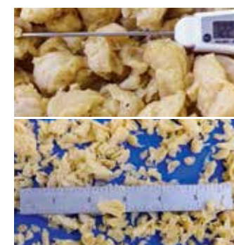
Pea Protein Extrusion 1/4" (6.4 mm) Shred, Sprint 2 Dicer
